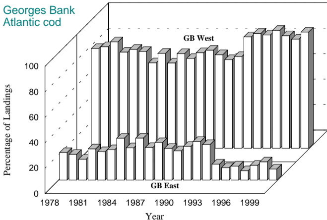
Figure 3. USA commercial landings of Georges Bank cod (NAFO Division 5Z and Subarea 6) for Eastern Georges Bank (SA 561-562) and Western Georges Bank (SA 521-522,525-526, 537-539, and Subarea 6), 1978-2000.
