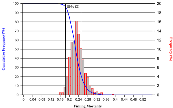
Figure 21. Precision of the estimates of the instantaneous rate of fishing ( F ) on the fully recruited ages (4+) in 2000 for Georges Bank cod. The bar height indicates the probability of values within that range. The solid line gives the probability that F is greater than any selected value on the X-axis.
