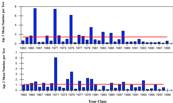
Figure 12. Relative year class strength of age 1 and age 2 Georges Bank cod based on standardized catch (number) per tow indices from NEFSC autumn research vessel bottom trawl surveys, 1963-2000. Horizontal line represents time series average.
